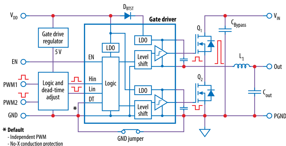
Figure 1: Block diagram of EPC9004C evaluation board
