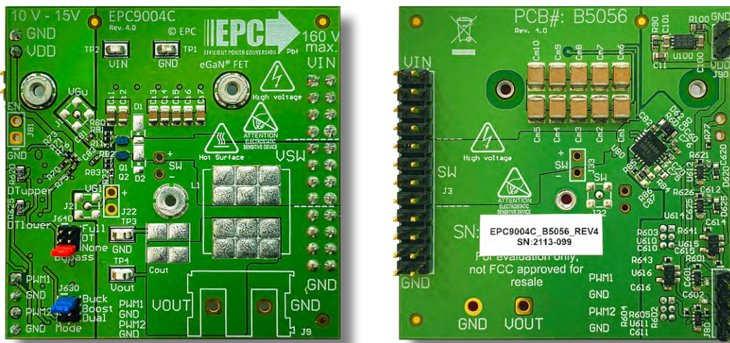
Front view EPC9004C evaluation board Back view
