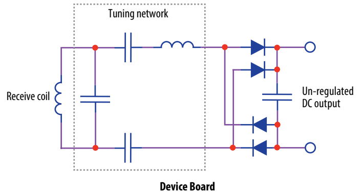
Figure 5: Schematic of Category 3 and Category 4 device board.
