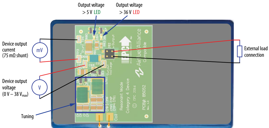
Figure 10: AirFuel Category 4 device board.
