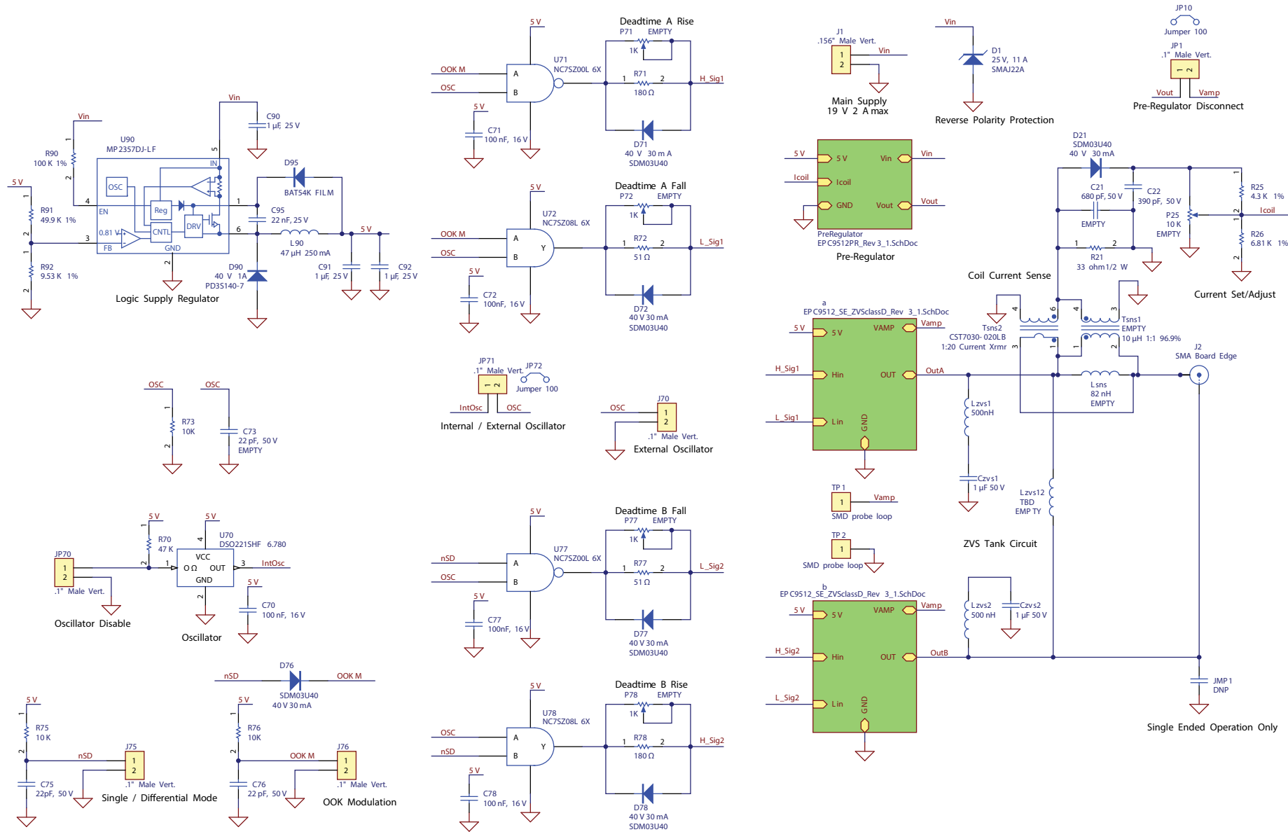
Figure 13: EPC9120 - ZVS class-D amplifier schematic.
