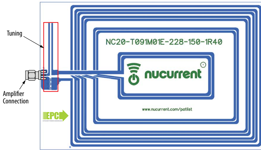
Figure 8: Proper connection for the source coil.
