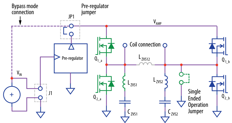
Figure 3: Diagram of EPC9512 ZVS class-D amplifier circuit.
