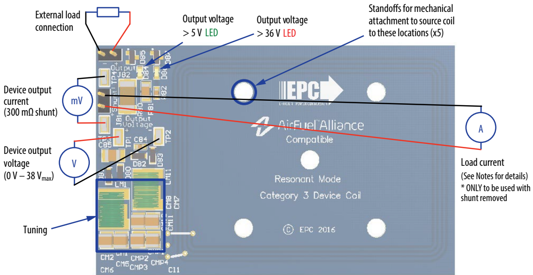
Figure 9: Proper connection and measurement for the Category 3 device coil.
