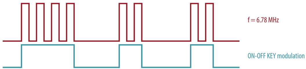
Figure 6: ON-OFF-KEY modulation.
