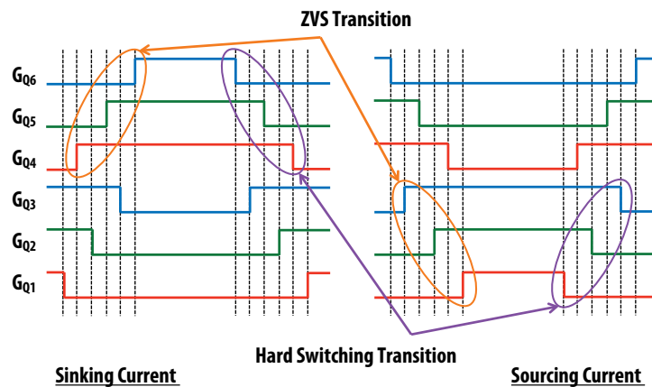
Figure 3 - Transistor switching sequencing
