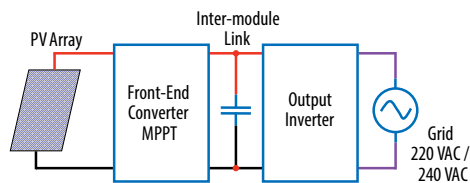
Figure 1: Simplified block diagram for a PV inverter
