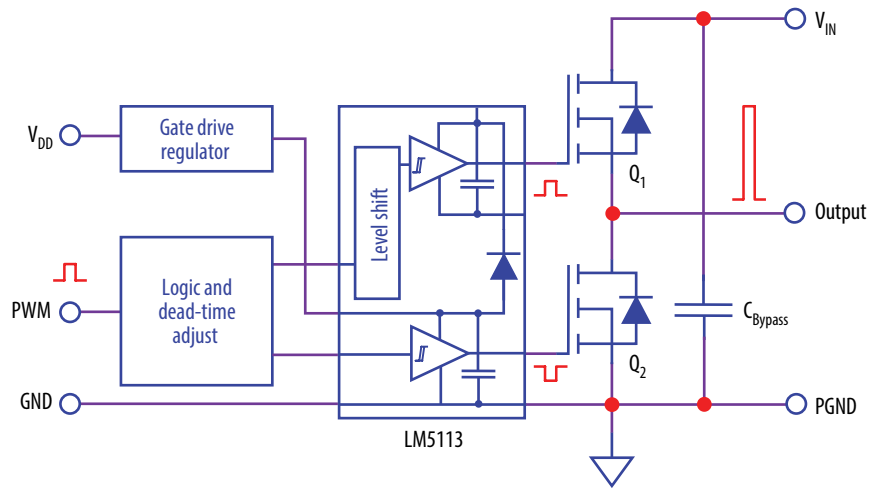
Figure 1: Block diagram of EPC9087 evaluation board.
