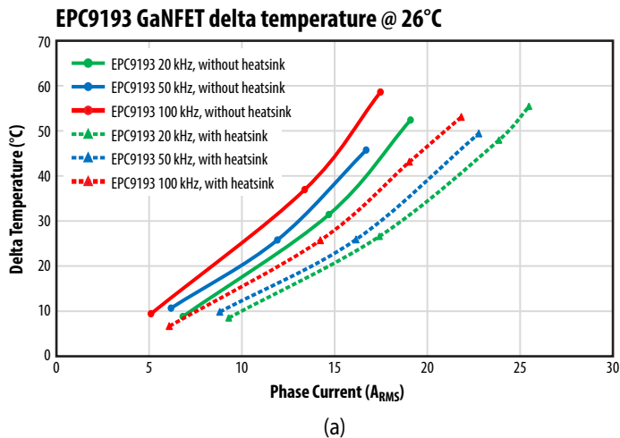
Figure 11: EPC9193 (a) and EPC9193HC (b) GaNFET temperature increase vs. the ambient temperature (26°C)
