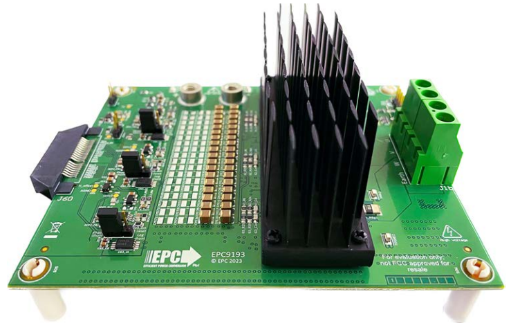
EPC9193 Evaluation board with heatsink attached
