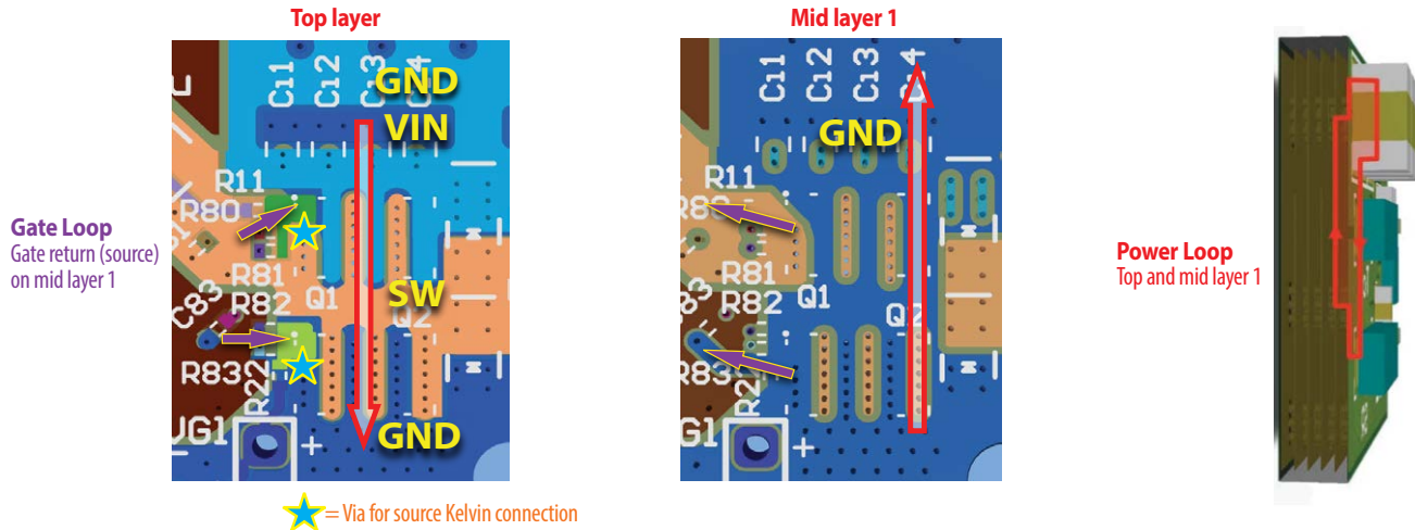
Figure 13: Inner vertical layout for power and gate loops from EPC90143
