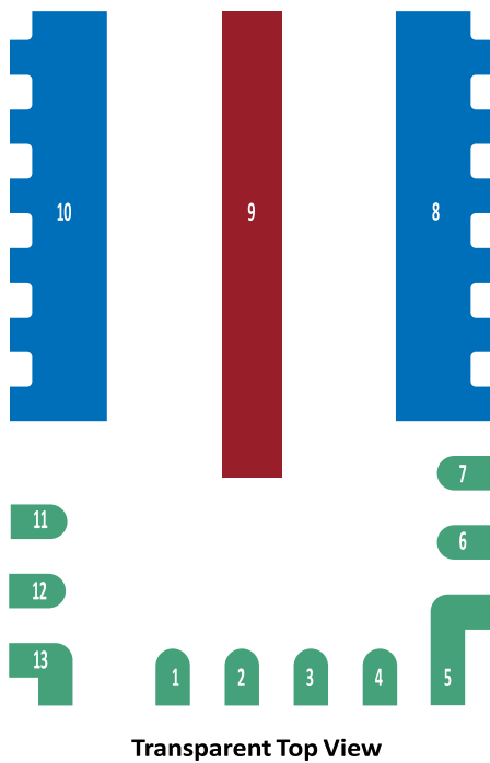
Figure 2: EPC23103 Quad Flat No-Lead (QFN) package (transparent top view)
