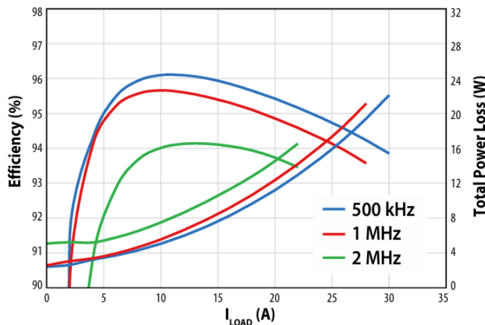
Figure 1: Performance curves
