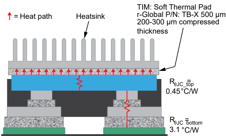
Figure 6: Parallel Thermal Resistance Paths of EPC23103 IC from junction to ambient
