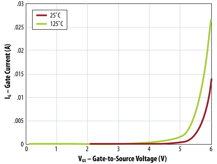
Figure 10: Gate Current
