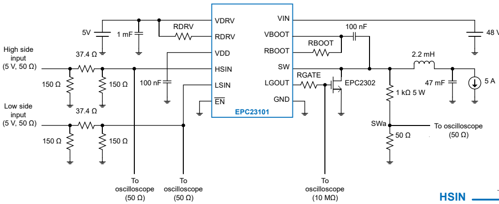
Figure 5a: Test Circuit for Dynamic Characteristics
