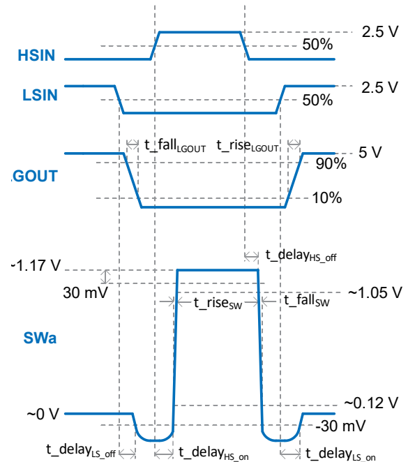
Figure 5b: Logic Input to Output Switching Node Timing Diagram
