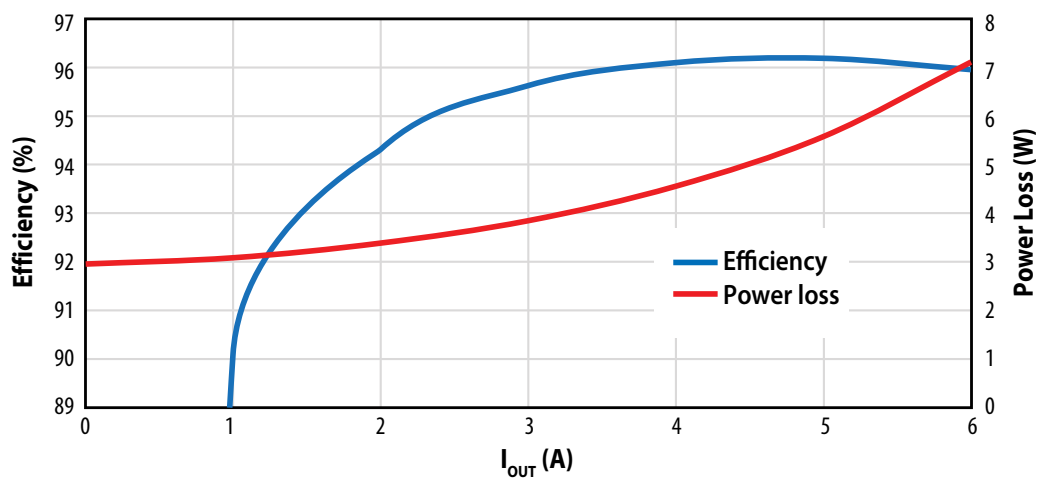
Figure 13: Measured efficiency and power loss operating from 280 V to 28 V at switching frequency 50 kHz and 47 \mu H inductance connected in series
