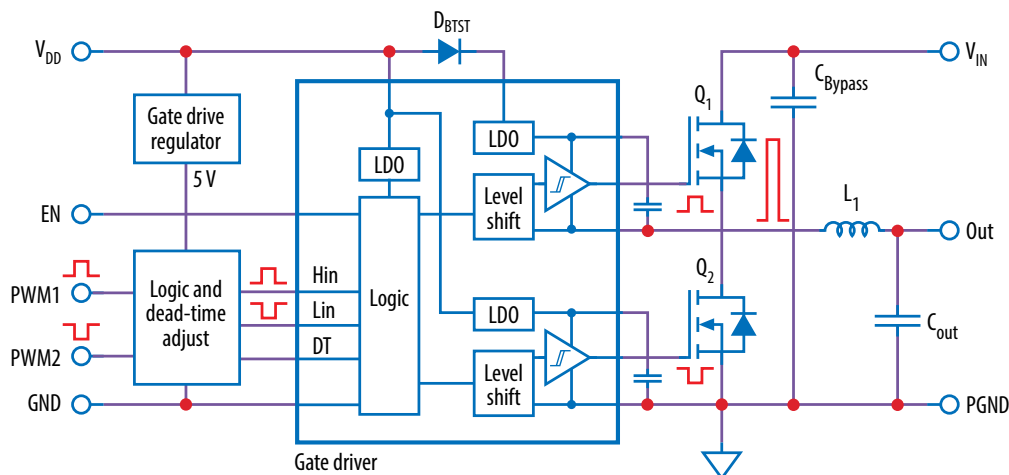
Figure 1: Block diagram of EPC90121 evaluation board
