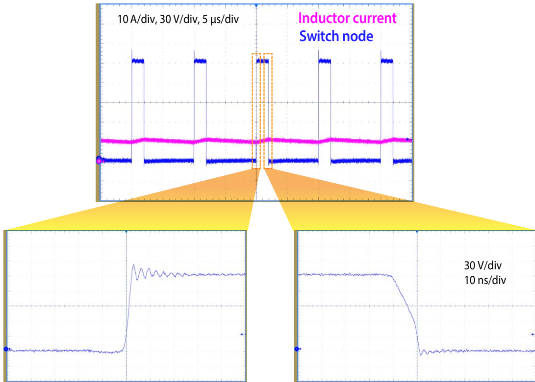
Figure 14: Measured inductor current and switch node waveforms when operating from 150 V at 100 kHz and delivering 10 A into a 30 V load
