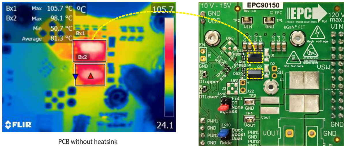
Figure 17: Measured thermal image and thermal couple readings of case temperature when operating under the following conditions: f_s = 100 kHz, I_{OUT} = 21 A output, 25°C ambient and moderate air flow
