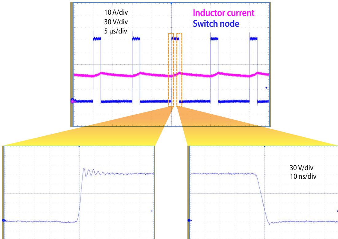
Figure 15: Measured inductor current and switch node waveforms when operating from 150 V at 100 kHz and delivering 30 A into a 21 V load
