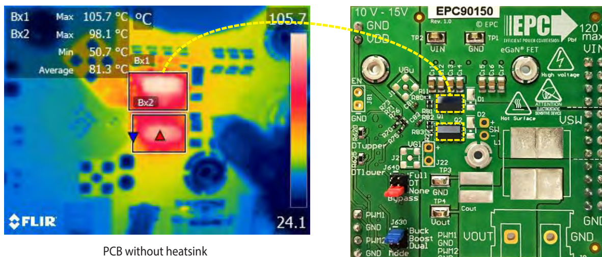
Figure 17: Measured thermal image and thermal couple readings of case temperature when operating under the following conditions: f_s = 100 \text{ kHz} , I_{OUT} = 21 \text{ A} output, 25^\circ\text{C} ambient and moderate air flow
