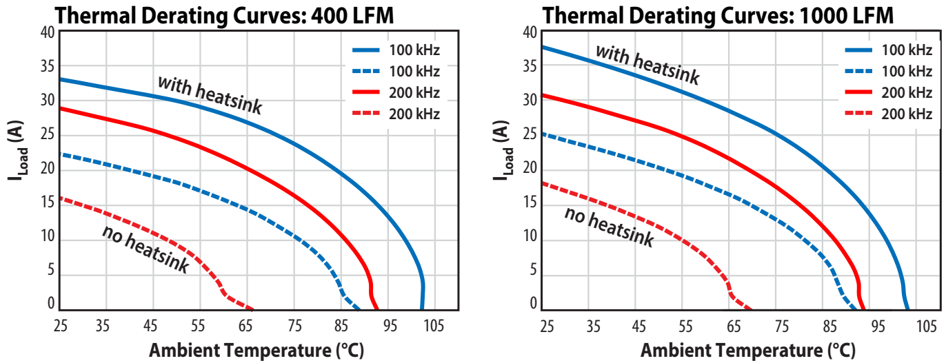
Figure 18: Typical thermal derating curve for two air flow rates, with and without a heatsink attached, measured with the board operating at various switching frequencies and using a 47 \mu H inductor
