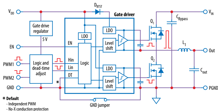
Figure 1: Functional block diagram overview of the EPC90150 board
