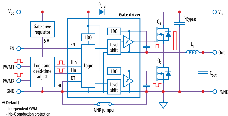
Figure 1: Functional block diagram overview of the EPC90150 board
