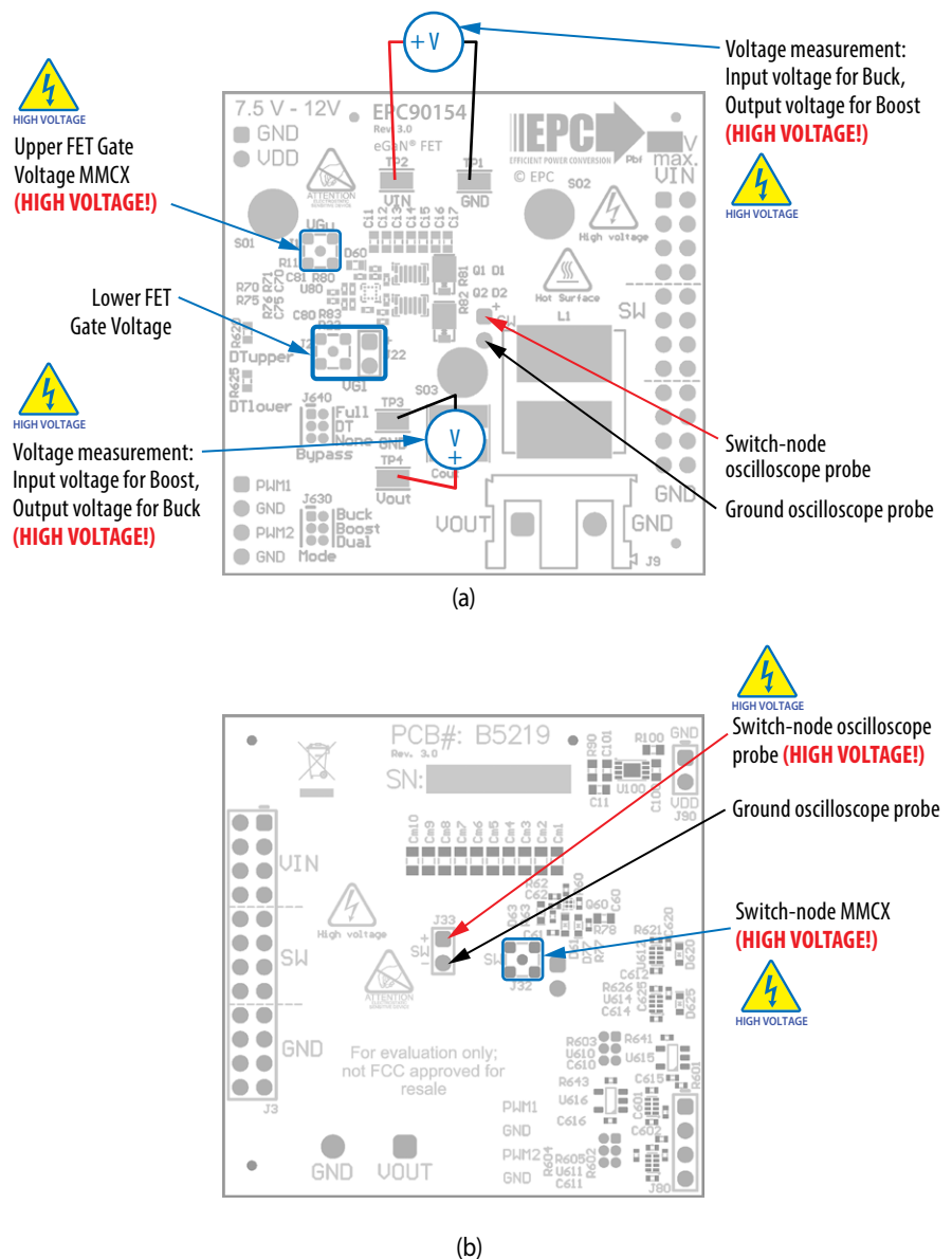
Figure 8: Measurement points (a) top side, (b) bottom side
