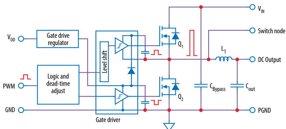
Figure 1: Block diagram of EPC90154 evaluation board default configuration
