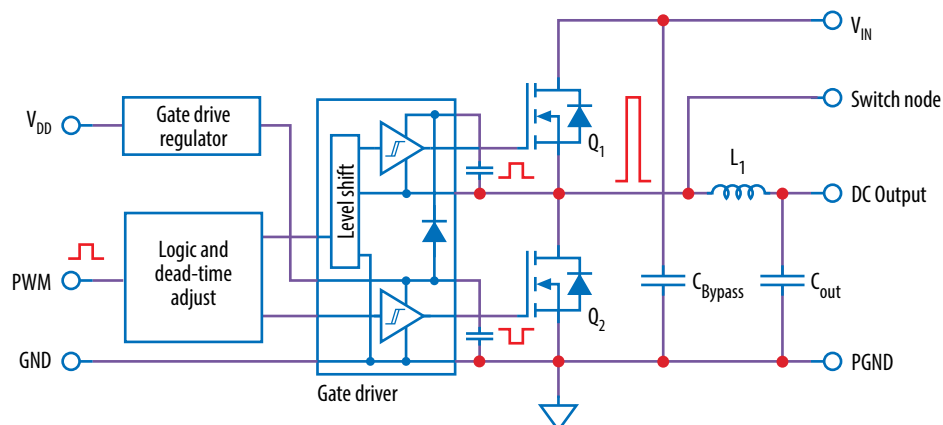
Figure 1: Block diagram of EPC90155 evaluation board default configuration
