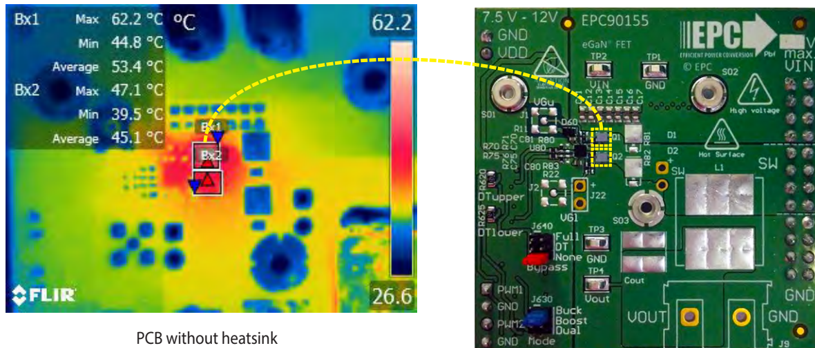
Figure 16: Measured thermal image and thermal couple readings of case temperature when operating under the following conditions: f_s = 1 \text{ MHz} , I_{OUT} = 7 \text{ A} output, 25^\circ\text{C} ambient and moderate air flow
