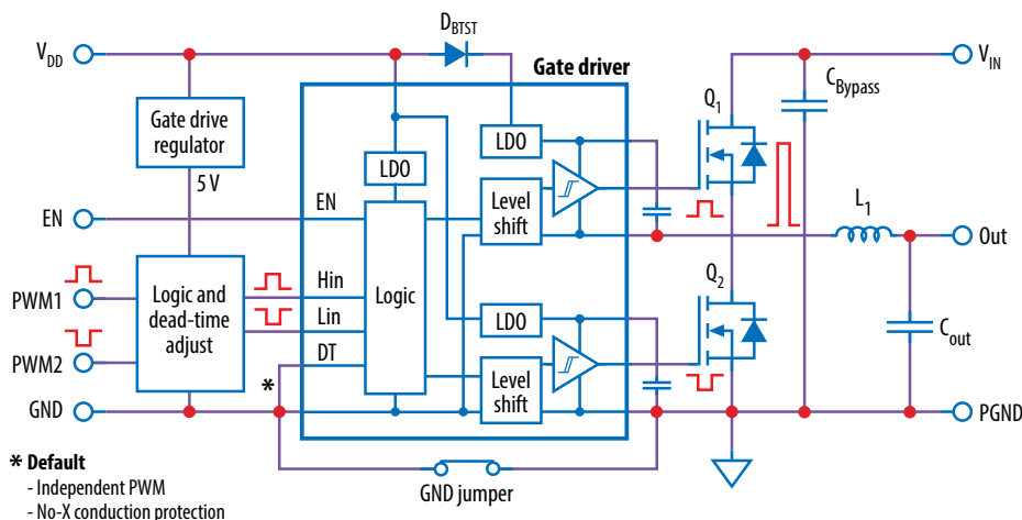
Figure 1: Block diagram of EPC9094 evaluation board
