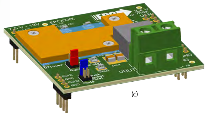
Figure 12: Details for attaching a heatsink to the evaluation board. (a) 3D perspective, (b) top view details, (c) Assembled view with heat-spreader attached.
