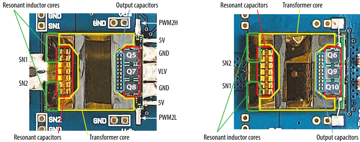
Figure 5: Zoomed-in photo of the EPC9551T transformer module with various components highlighted
