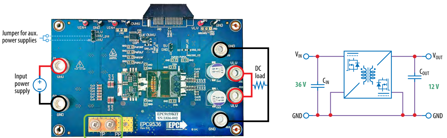
Figure 7: Left: Power connections and configuration for operation in Through Power Mode. Right: Block diagram of the converter in Through Power Mode.
