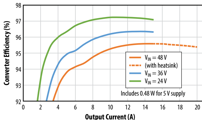
Figure 11: Measured efficiency, including the effect of control power, of the EPC9177 board operating in buck mode for multiple input voltages and V_{OUT} = 12\text{ V} , 400 LFM airflow and without a heatsink. Dashed line shows the extended load current range when using a heatsink
