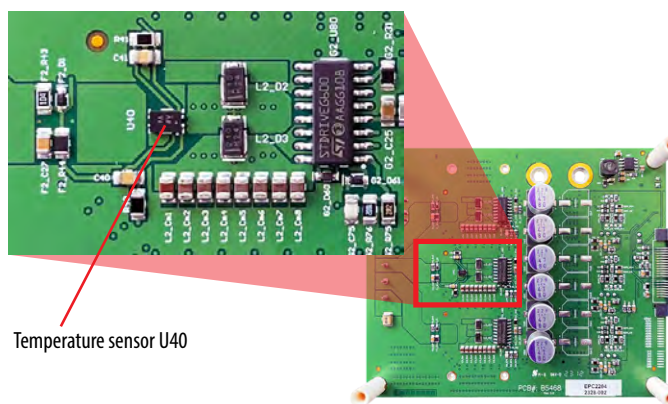
Figure 13: Temperature sensor location on the bottom side of the PCB
