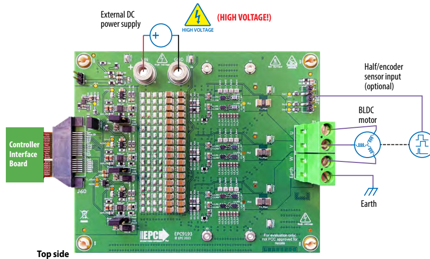
Figure 5: Connection diagram of the EPC9193 configured as a motor drive inverter
