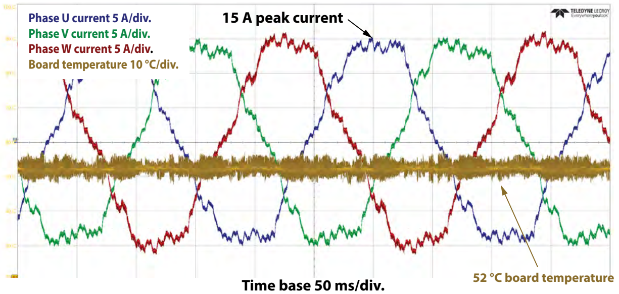
Figure 9. Phase current waveforms and board temperature
