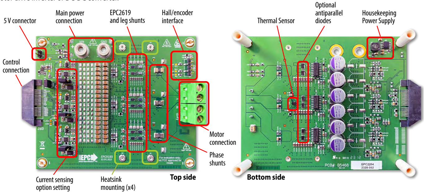
Figure 1: Photo overview of the EPC9193HC board highlighting the main sections
