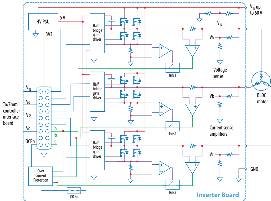
Figure 2. Block diagram of EPC9193HC board in BLDC drive example application
