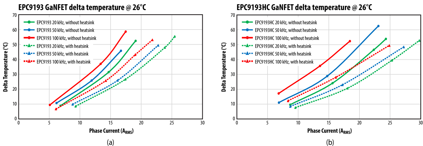
Figure 11: EPC9193 (a) and EPC9193HC (b) GaNFET temperature increase vs. the ambient temperature (26°C)
