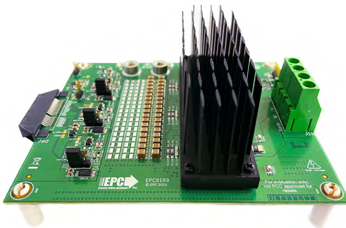
EPC9193 Evaluation board with heatsink attached
