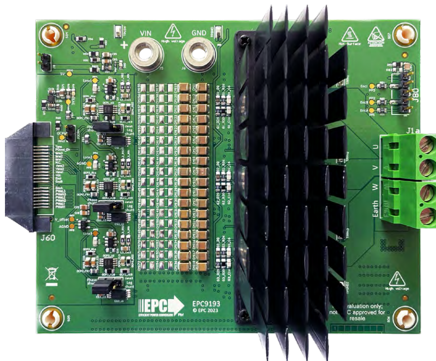
Figure 8: Natural convection cooling heatsink installed on the EPC9193 inverter board
