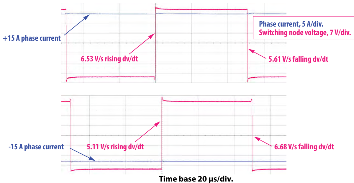
Figure 10. Measured slew rate on rising and falling switch-node transitions at 15 A peak positive and negative phase current
