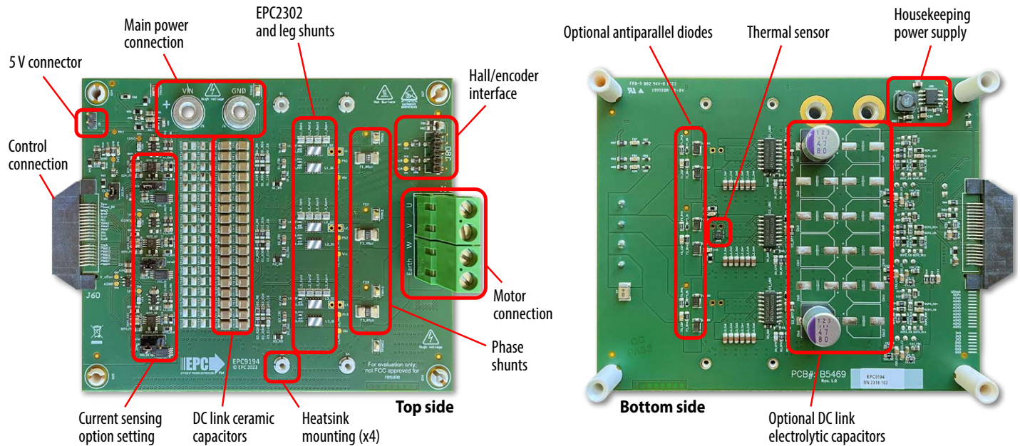
Figure 1: Photo overview of the EPC9194 board highlighting the main sections
