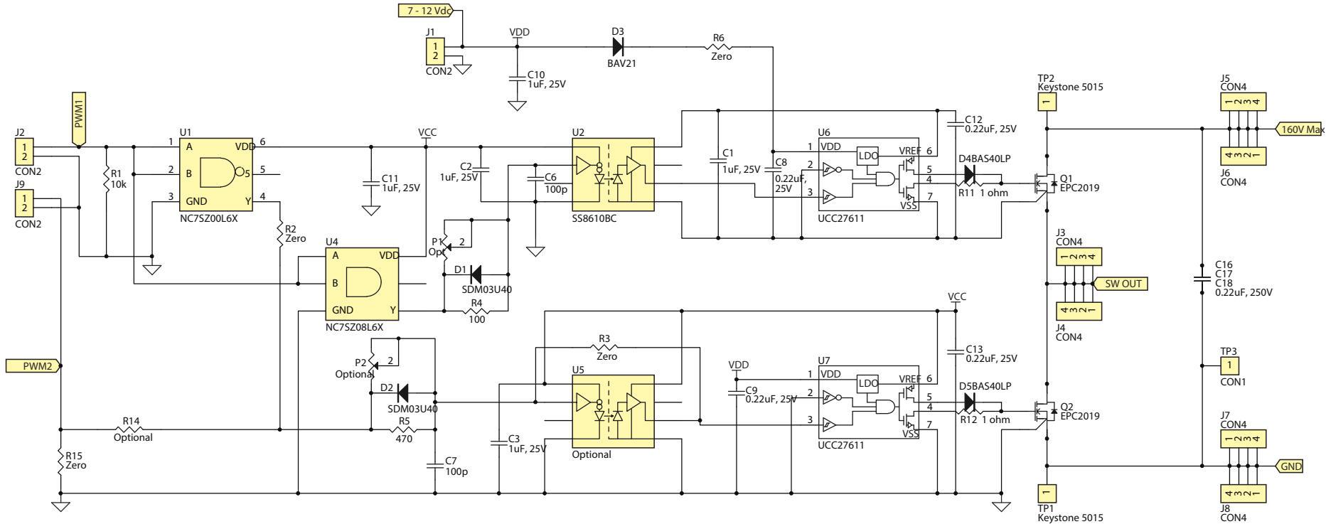
EPC9014 200V Half-Bridge with Gate Drive, using EPC2019 Rev 1.0
