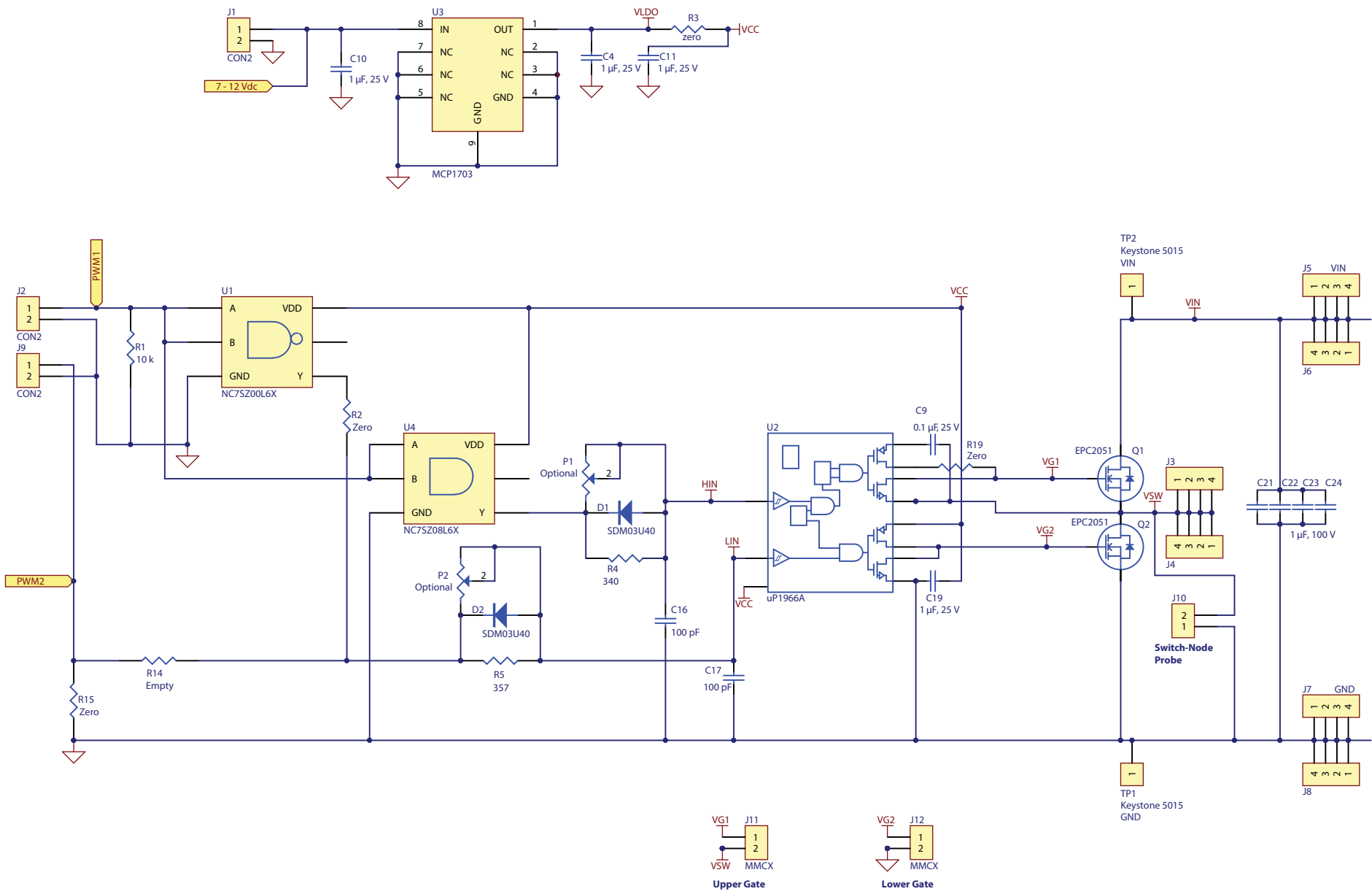
Figure 4: EPC9091 - Schematic
