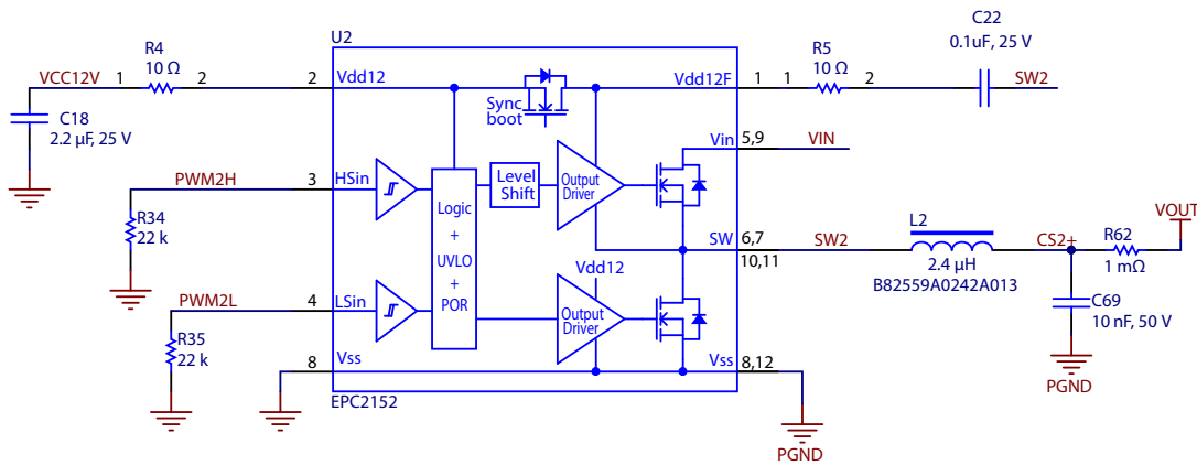
Figure 20: EPC9151 Power Stage schematic
