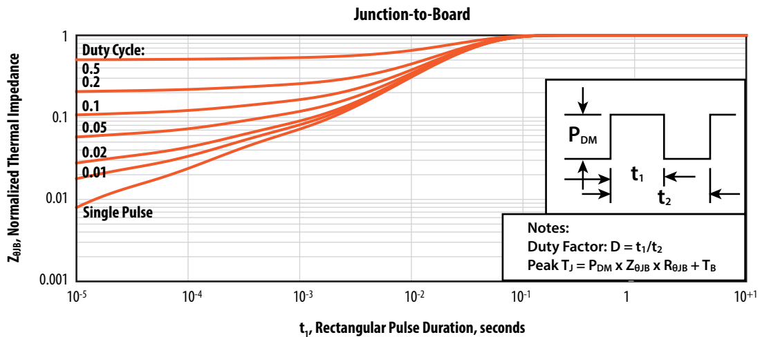
Figure 12: Typical Transient Thermal Response Curves
