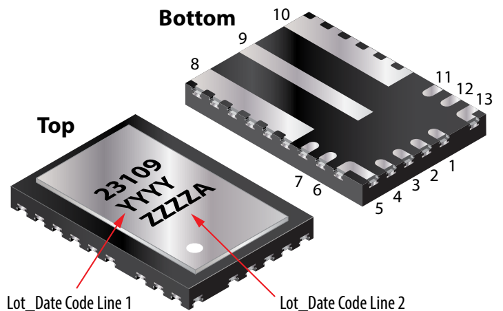
Figure 8: EPC23109 QFN package outline, pinouts and exposed backside of the GaN IC die
