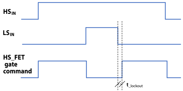
Figure 19: Cross-Conduction Logic Timing Diagram
