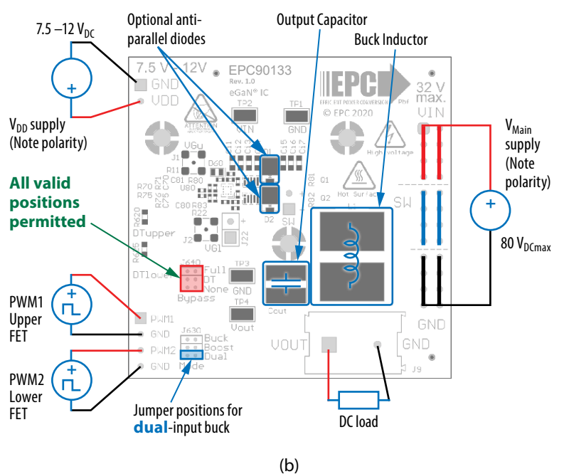
Figure 6: (a) Single-PWM input buck converter (b) Dual-PWM input buck converter configurations showing the supply, anti-parallel diodes, output capacitor, inductor, PWM, and load connections with corresponding jumper positions.
