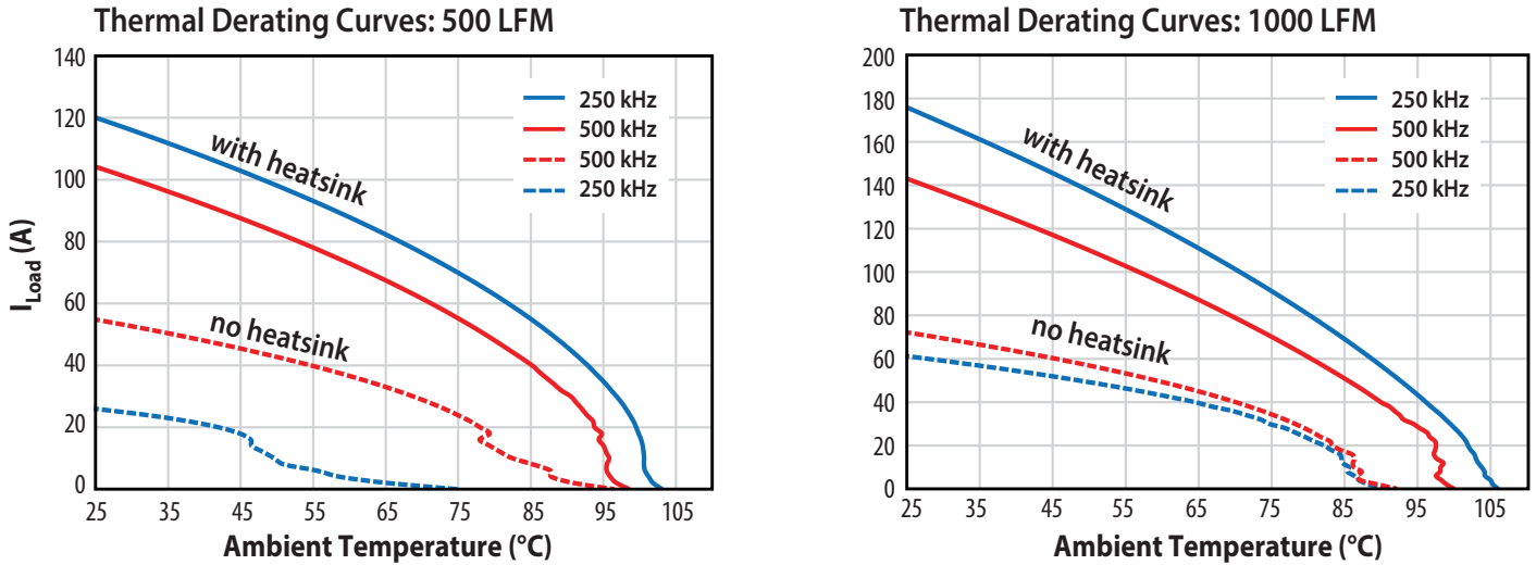
Figure 16: Typical thermal derating curve for two air flow rates, with and without a heatsink attached, measured with the board operating at various switching frequencies and using a 2.2 μH inductor
