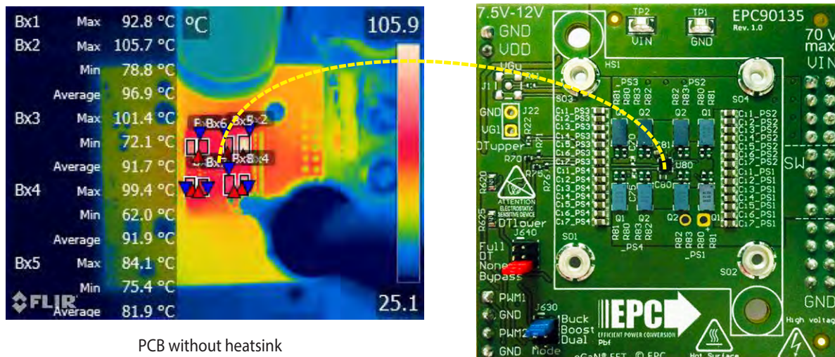
Figure 15: Measured thermal image and thermal couple readings of case temperature when operating under the following conditions: f_s = 500 \text{ kHz} , I_{OUT} = 55 \text{ A} output, 25°C ambient and high air flow
