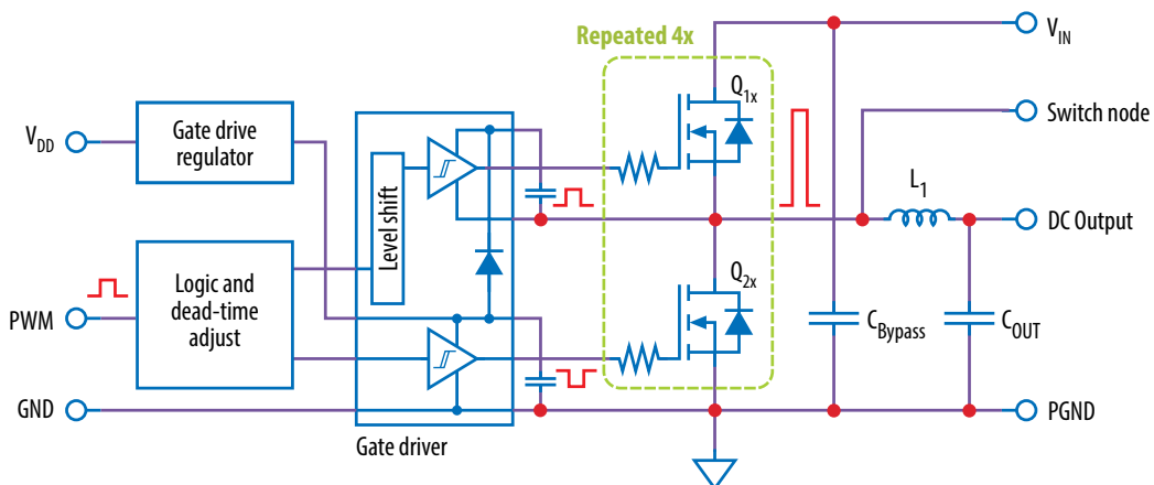
Figure 1: Block diagram of EPC90135 evaluation board default configuration
