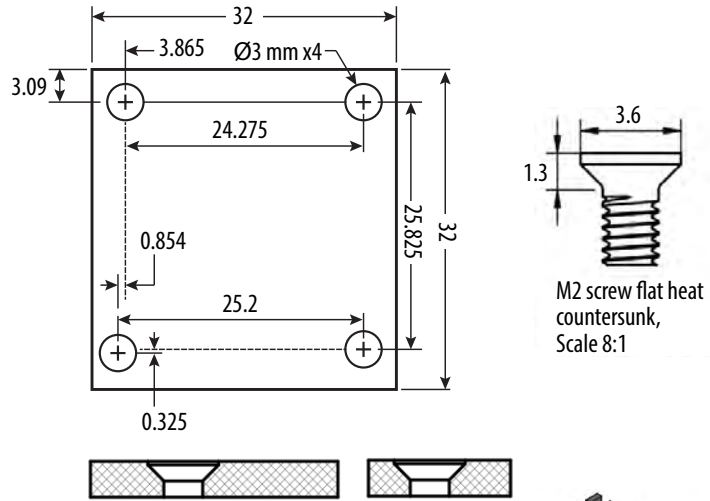
Figure 9: Heat-spreader details
