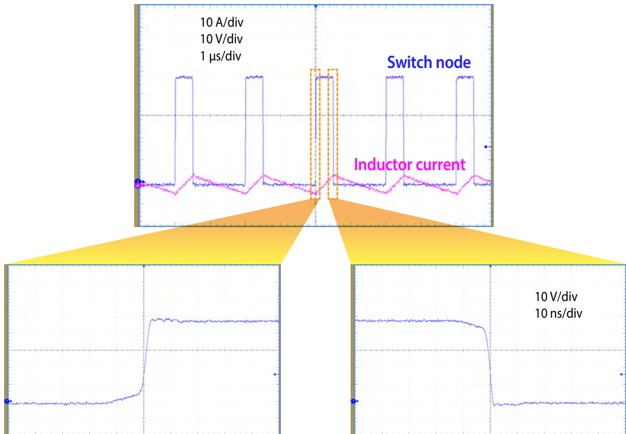
Figure 11: Measured inductor current and switch node waveforms when operating from 48 V at 500 kHz and delivering 0 A into a 12 V load
