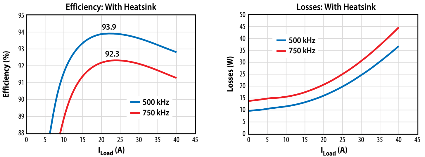
Figure 14: Measured efficiency and power loss operating at various switching frequencies and using L = 2.2 \mu H
