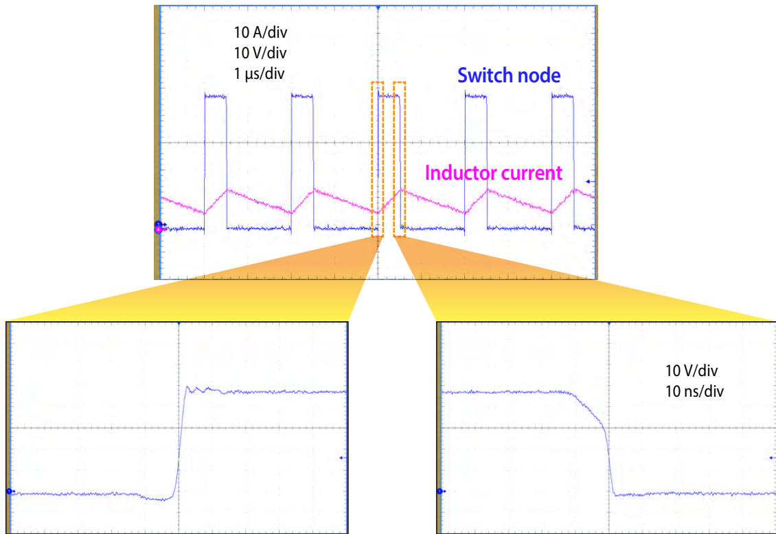
Figure 12: Measured inductor current and switch node waveforms when operating from 48 V at 500 kHz and delivering 10 A into a 12 V load
