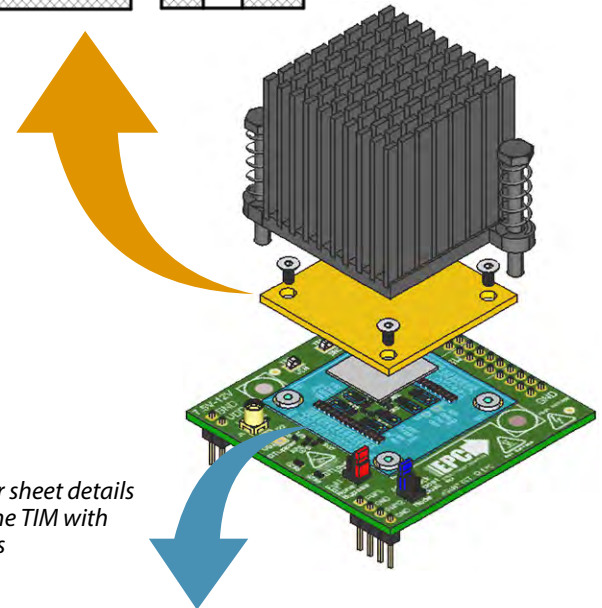
Figure 9: Heat-spreader details
