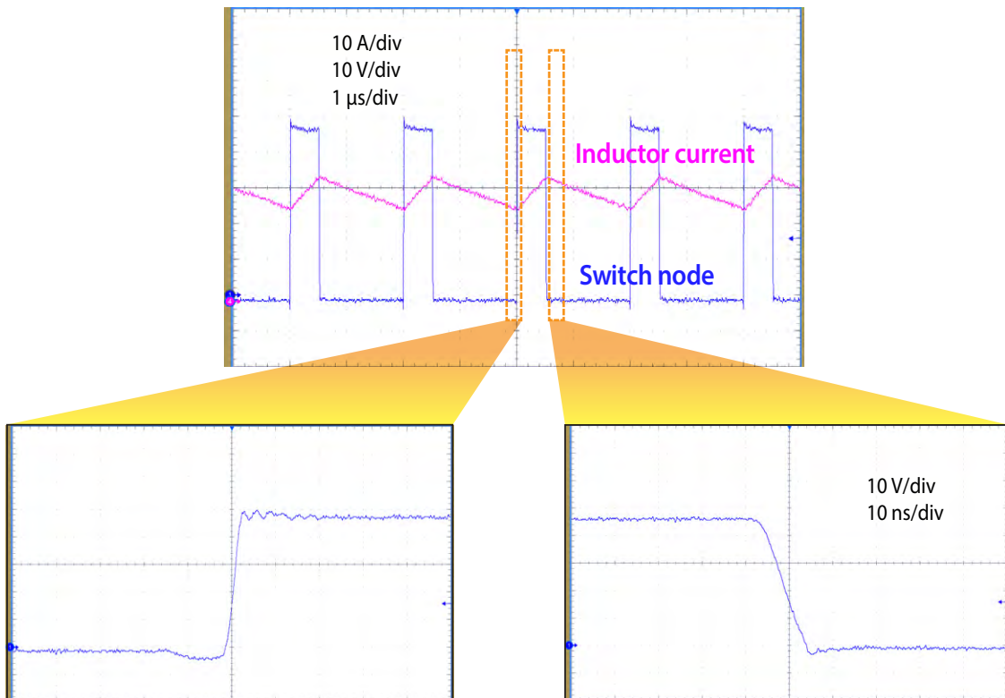
Figure 13: Measured inductor current and switch node waveforms when operating from 48 V at 500 kHz and delivering 30 A into a 12 V load
