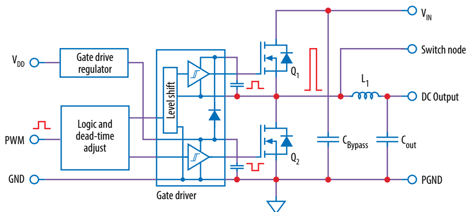
Figure 1: Block diagram of EPC90138 evaluation board default configuration
