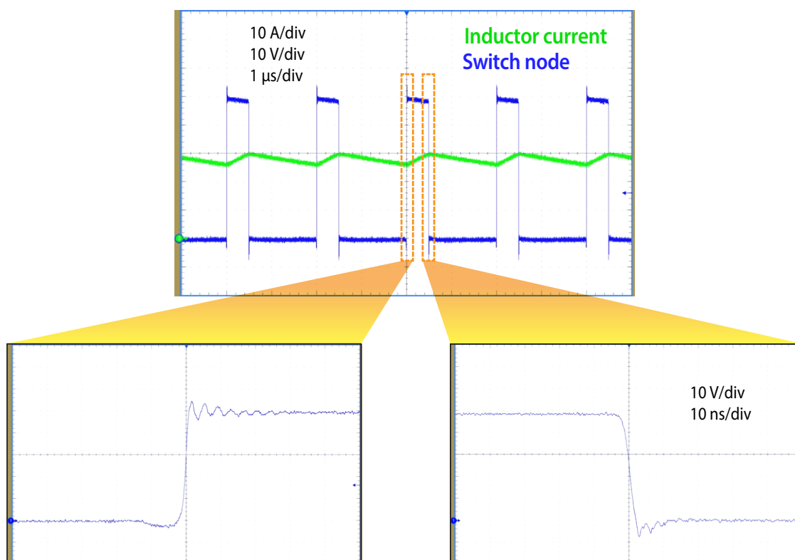
Figure 14: Measured inductor current and switch node waveforms when operating from 48 V at 500 kHz and delivering 28 A into a 12 V load
