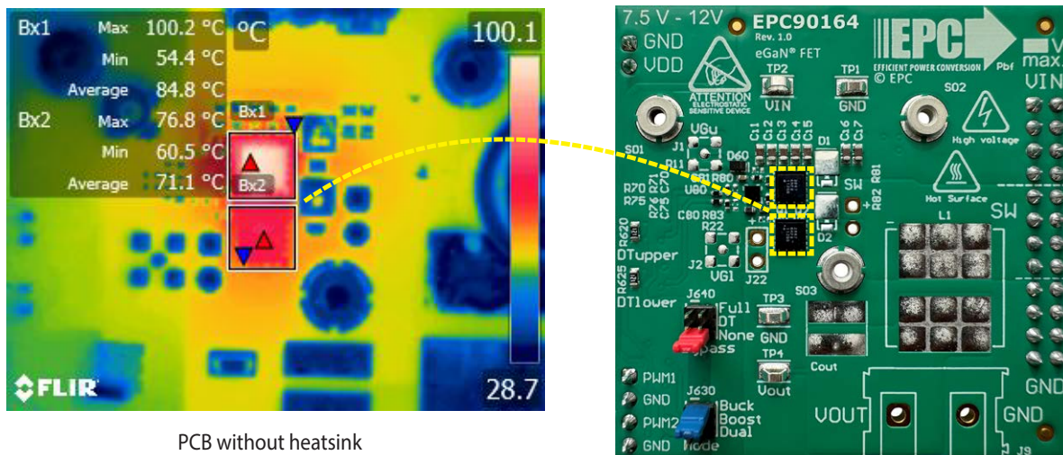
Figure 16: Measured thermal image reading of case temperature when operating under the following conditions: f_s = 500 \text{ kHz} , I_{OUT} = 28 \text{ A} output, 25^\circ\text{C} ambient and high air flow
