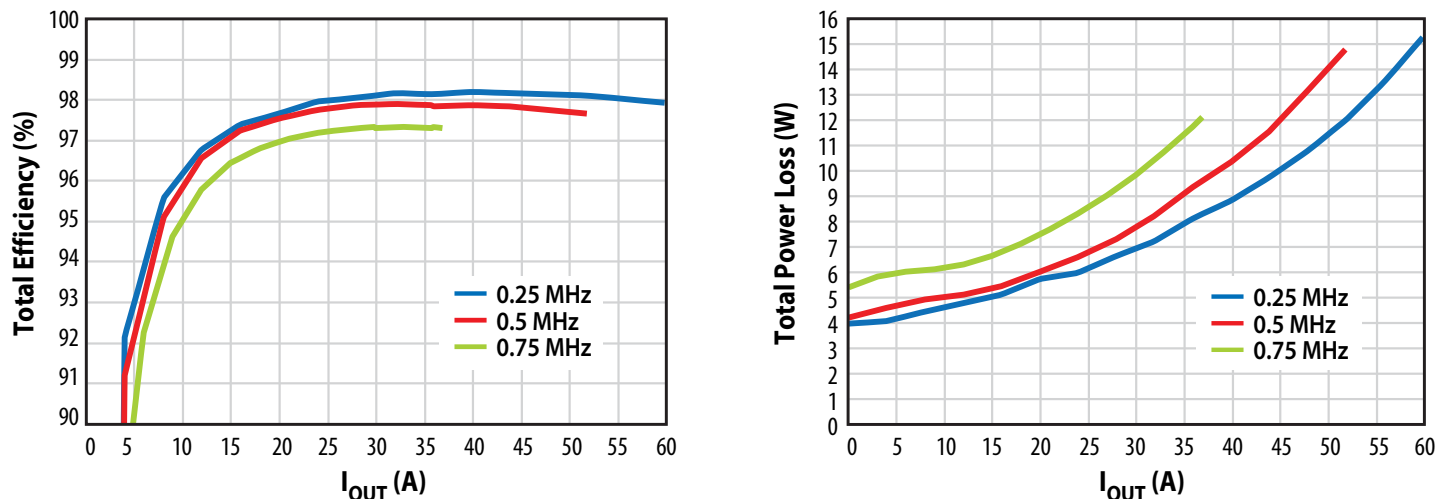
Figure 16: Measured efficiency at 48 V IN , 12 V OUT , across various switching frequencies, up to a maximum output current that results in 100°C of case temperature
