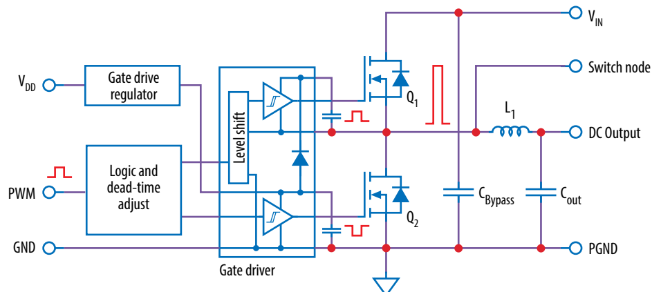
Figure 1: Block diagram of EPC90189 evaluation board default configuration
