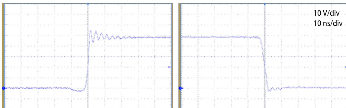
Figure 14: Measured switchnode voltage at 48 V IN , 12 V OUT , 0.5 MHz, 26 A
