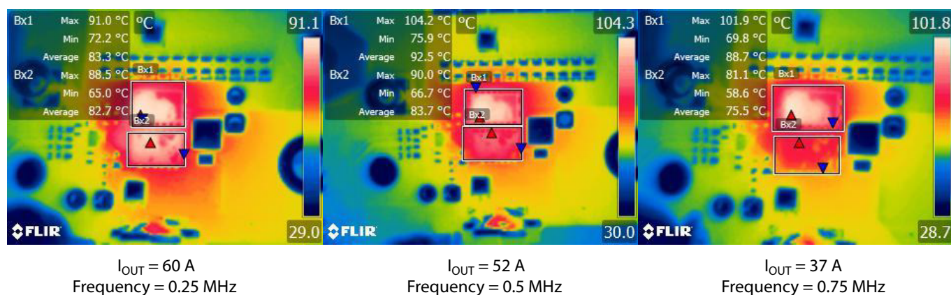
Figure 19: Thermal images of EPC90189 operating at 48 V IN , 12 V OUT , maximum current required to reach 100°C, across various switching frequencies with 25°C ambient temperature
