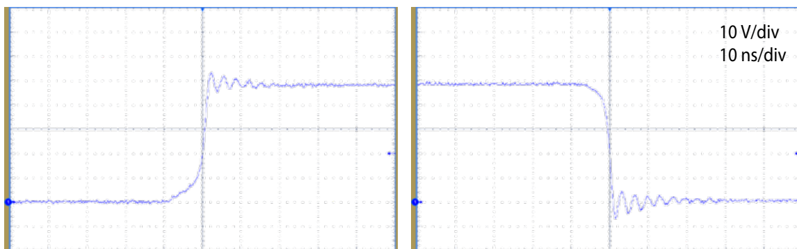
Figure 13: Measured switchnode voltage at 48 V IN , 12 V OUT , 0.5 MHz, 0 A
