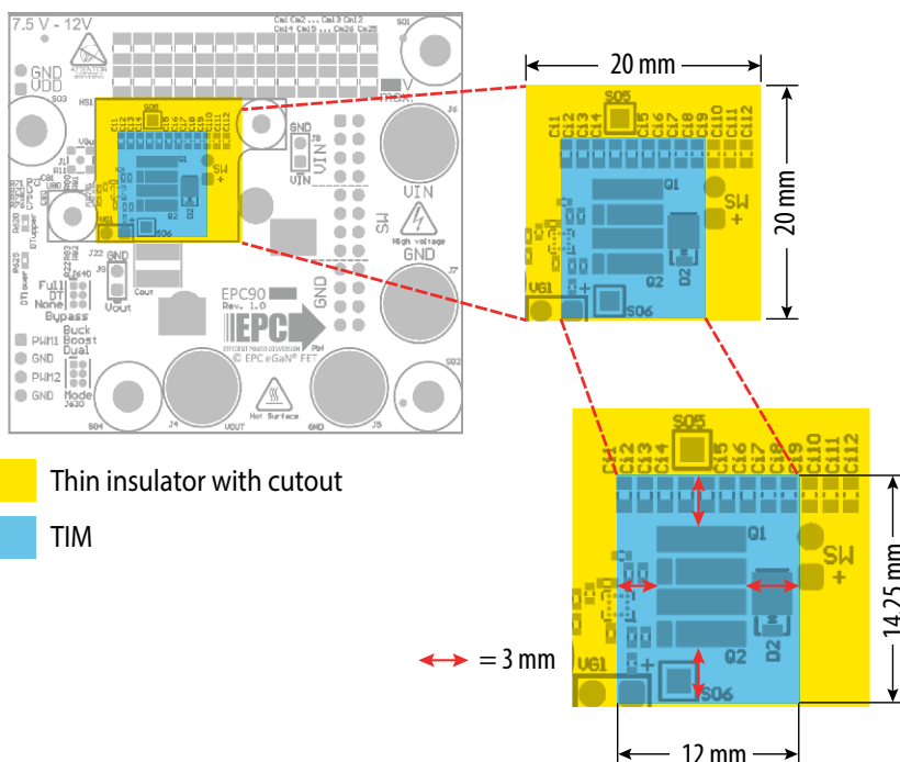
Figure 12: Alternative TIM configuration with insulator sheet with cutout for the TIM
