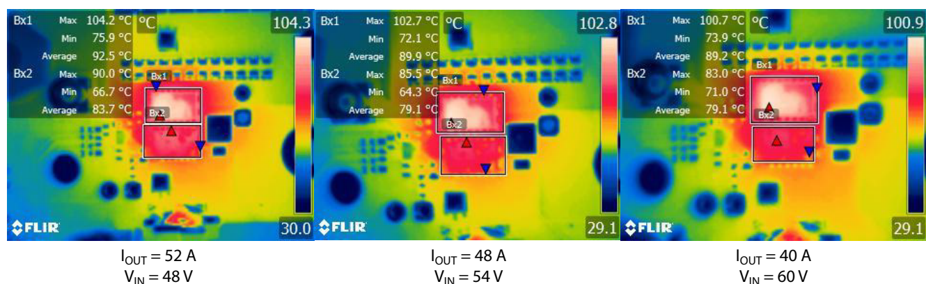
Figure 18: Thermal images of EPC90189 operating at 0.5 MHz and 12 V OUT with 25°C ambient temperature
