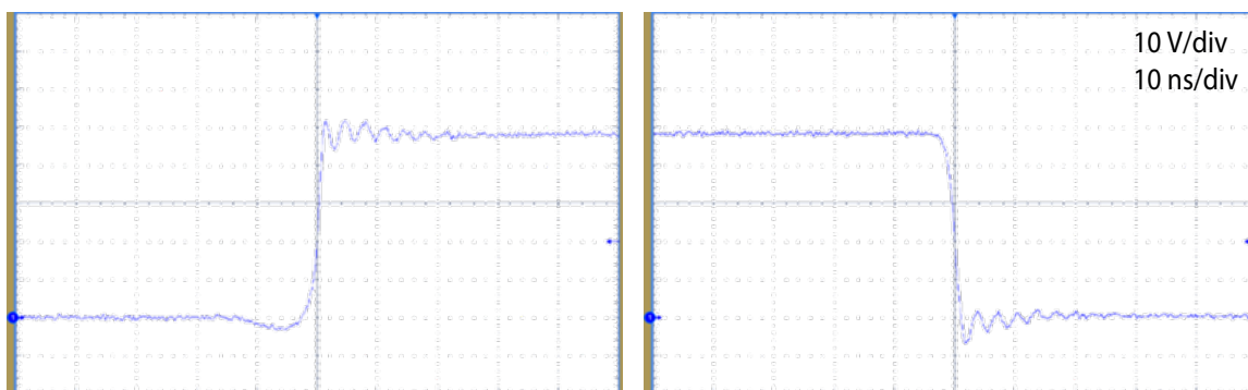
Figure 15: Measured switchnode voltage at 48 V IN , 12 V OUT , 0.5 MHz, 52 A
