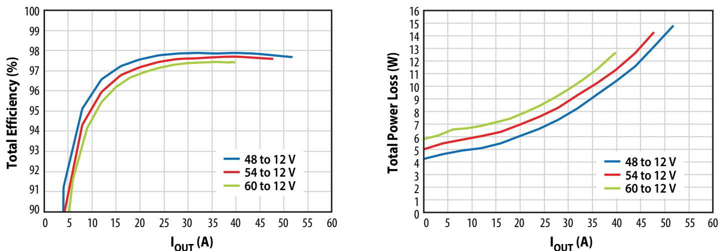
Figure 17: Measured efficiency at 0.5 MHz, 12 V OUT , across various input voltages, up to a maximum output current that results in 100°C of case temperature
