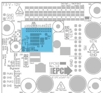
Figure 11: Size and location of the TIM
