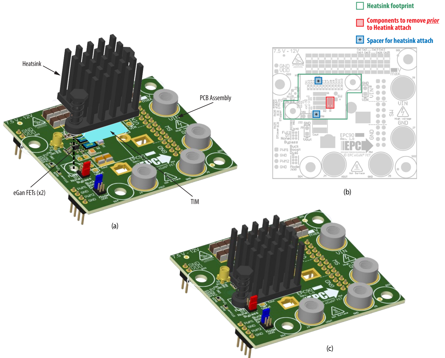
Figure 10: Details for attaching a heatsink to the evaluation board.
