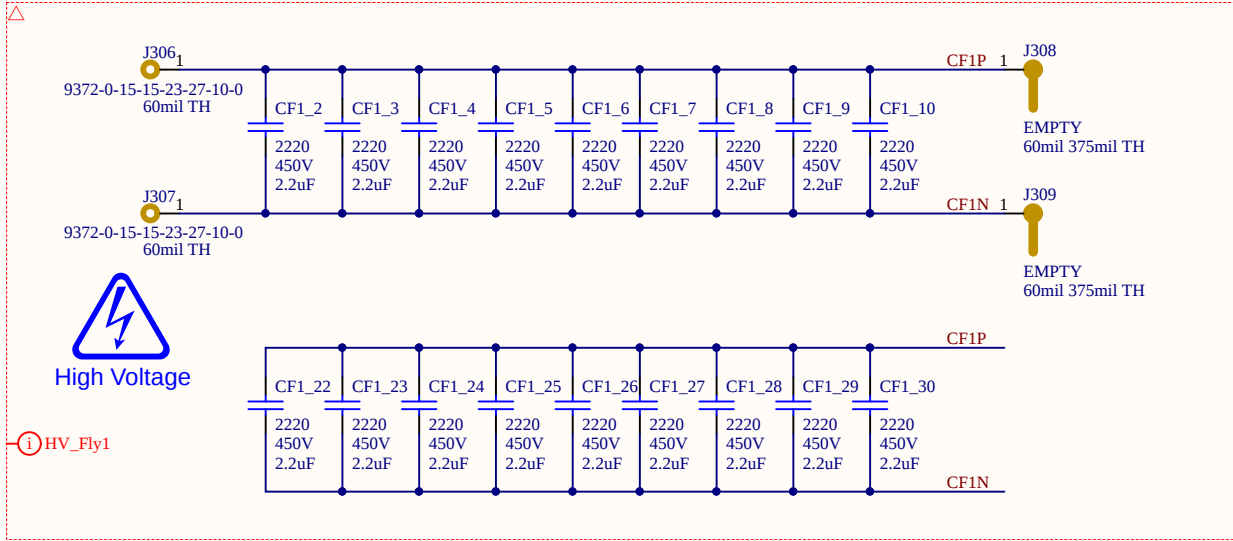
Extra Capacitor Bank
