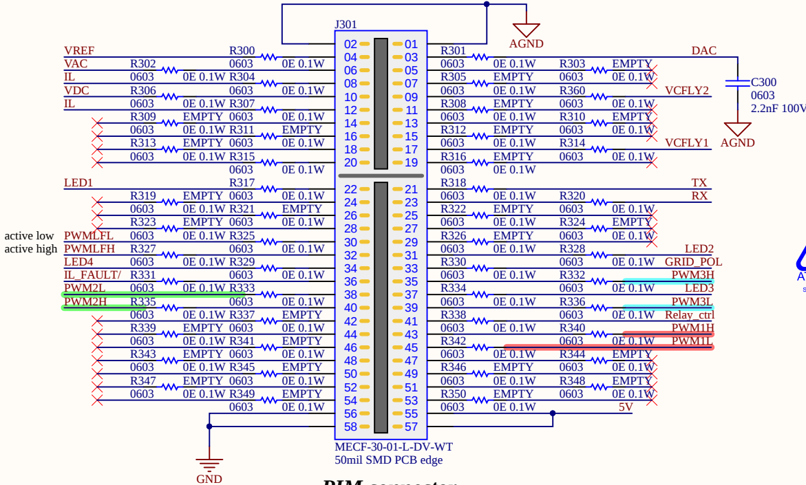
PIM connector
