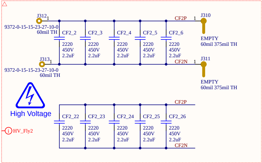
Main Capacitor Bank
