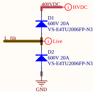
Pre-charge Diodes
