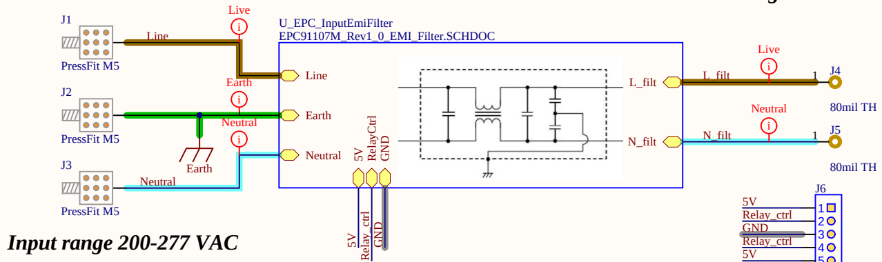
EMI Filter and In-rush relay
