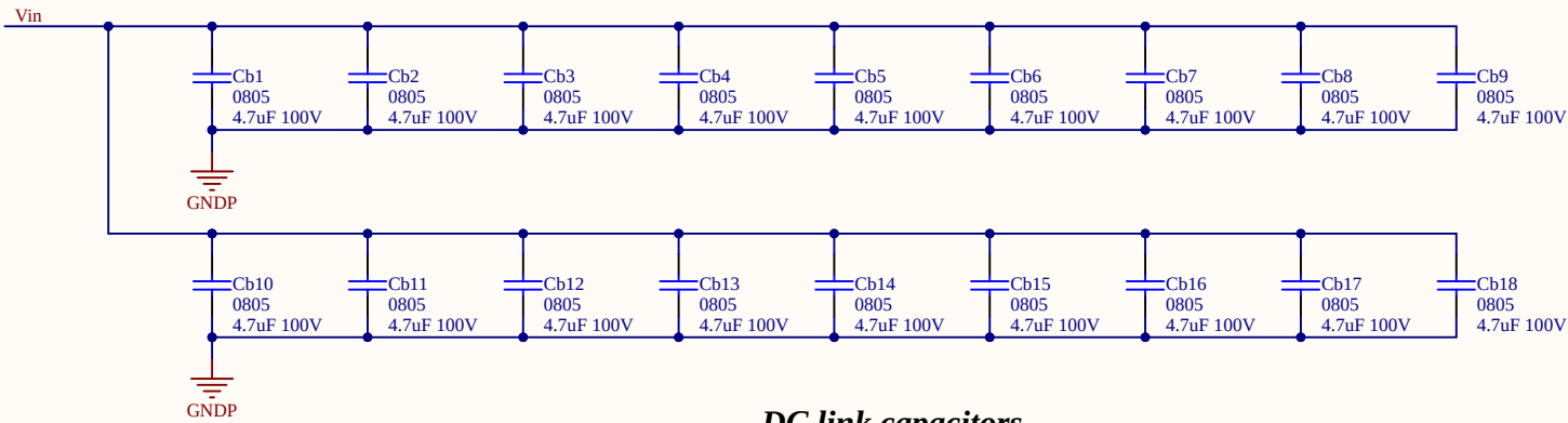
DC link capacitors
