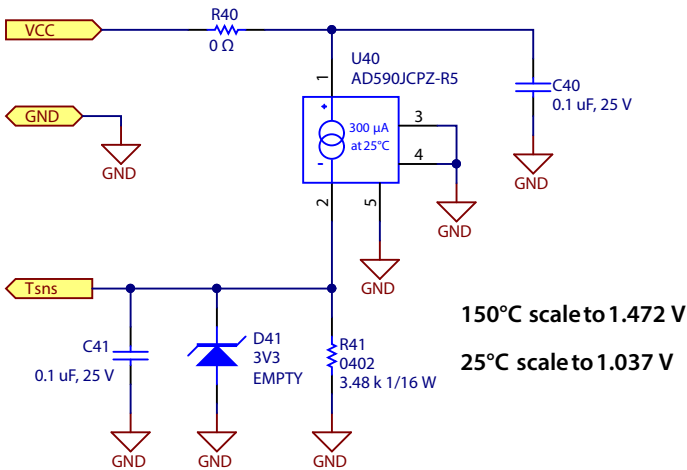
Figure 21: EPC9163 AD590 temperature sense schematic
