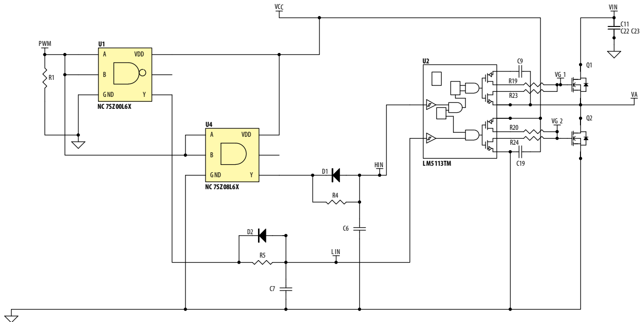
Development Board Schematic Rev 0
