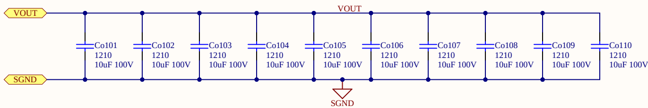
Output Bus Capacitance
