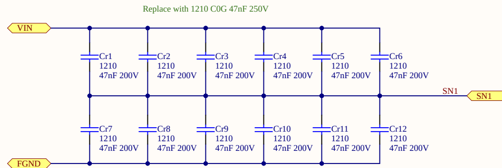
Resonant capacitors
