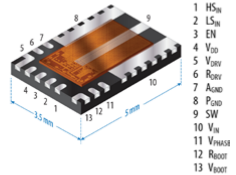
Figure 6: Detailed block diagram symbol and photo with pin assignments of the EPC23102.
