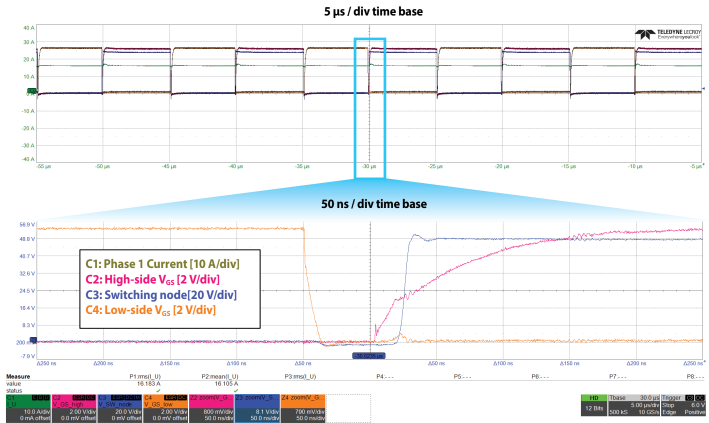
Figure 12: Phase waveforms during switching transitions
