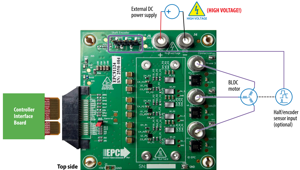
Figure 5: Connection diagram of the EPC91124 configured as a motor drive inverter
