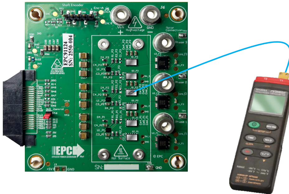
Figure 7: Thermal test setup configuration
