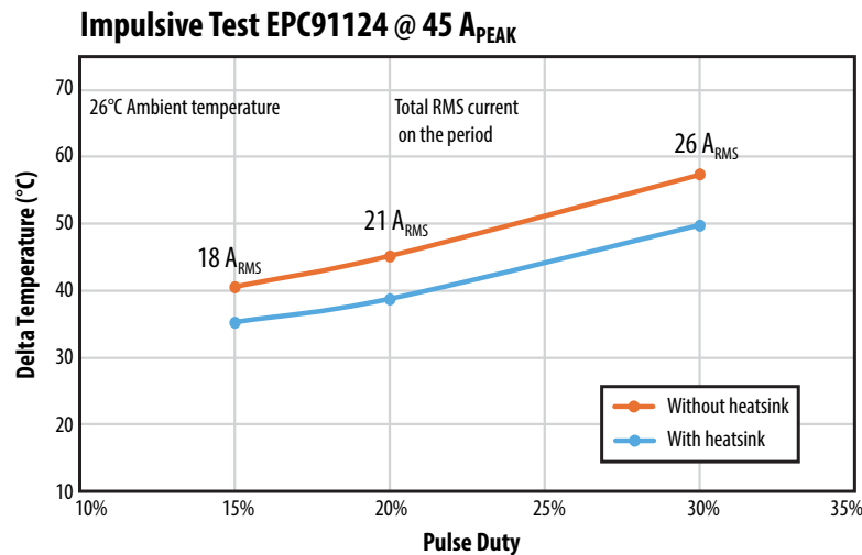
Figure 11: EPC91124 (EPC2361 eGaN® FET) temperature increases vs. ambient temperature (26°C).
