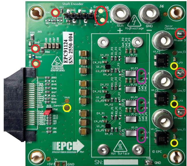
Figure 4: EPC91124 test point pad and hookup locations and designations in red. In black the GND reference points and in yellow the AGND reference point. In purple the 100 mils holes for the switching node measurements
