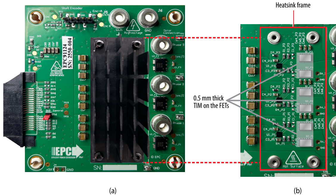
Figure 6: (a) passive heatsink mounted on EPC91124 board (b) details on TIM placement
