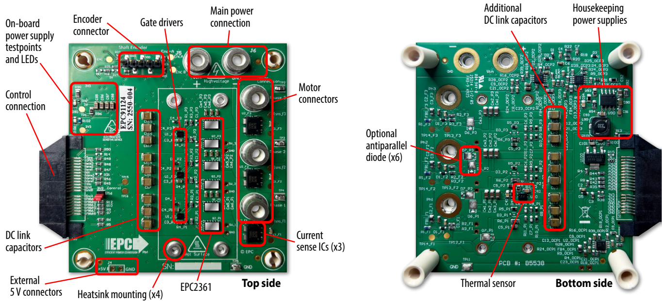
Figure 1: Photo overview of the EPC91124 board highlighting the main sections
