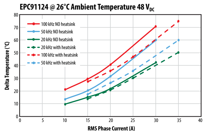
Figure 8: EPC91124 (EPC2361 eGaN® FET) temperatures increase vs. the ambient temperature (26°C). Measurements were taken at various PWM frequencies
