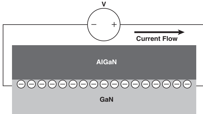
Figure 1.4 By applying a voltage to the 2DEG an electric current is induced in the crystal
