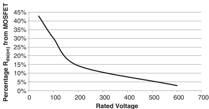
Figure 1.12 At a higher voltage rating the low voltage MOSFET does not add significantly to the on-resistance of the cascode transistor system
