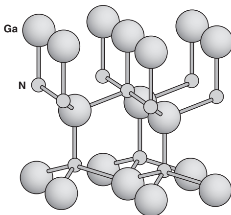
Figure 1.2 Schematic of wurtzite GaN
