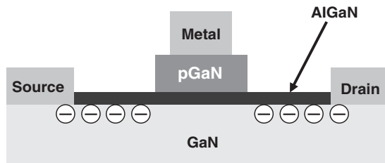
Figure 1.10 By growing a p-type GaN layer on top of the AlGaN the 2DEG is depleted at zero volts on the gate
