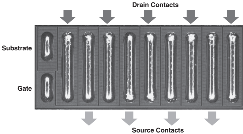
Figure 1.20 A finished device with solder bars in land grid array (LGA). This device measures approximately 4 mm × 1.6 mm
