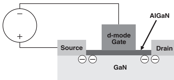
Figure 1.5 By applying a negative voltage to the gate of the device, the electrons in the 2DEG are depleted out of the device. This type of device is called a depletion-mode (d-mode) HEMT
