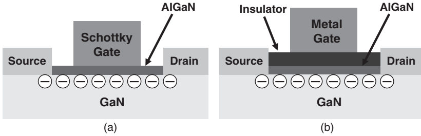
Figure 1.6 Cross section of a basic depletion-mode GaN HEMT with (a) Schottky gate, or (b) insulating gate
