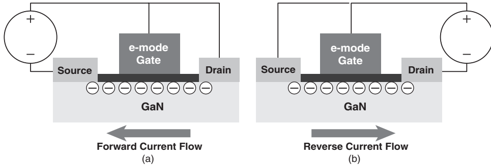
Figure 1.13 Enhancement-mode HEMT transistors can conduct in either the forward or reverse direction
