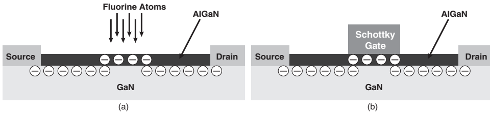
Figure 1.9 (a) By implanting fluorine atoms into the AlGaN barrier layer negative charges are trapped in the barrier. (b) A Schottky gate now can be used to reconstruct the 2DEG when a positive voltage is applied
