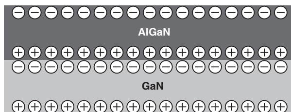
Figure 1.3 Simplified cross section of a GaN/AlGaIn heterostructure showing the formation of a 2DEG due to the strain-induced polarization at the interface between the two materials
