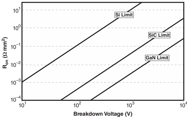
Figure 1.1 Theoretical on-resistance for a one square millimeter device vs. blocking voltage capability for Si, SiC, and GaN based power devices
