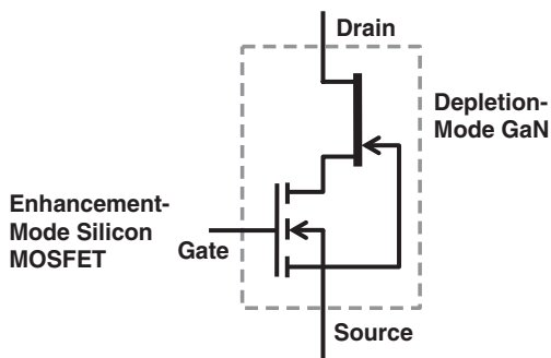
Figure 1.11 Schematic of low-voltage enhancement-mode silicon MOSFET in series with a depletion-mode GaN HEMT
