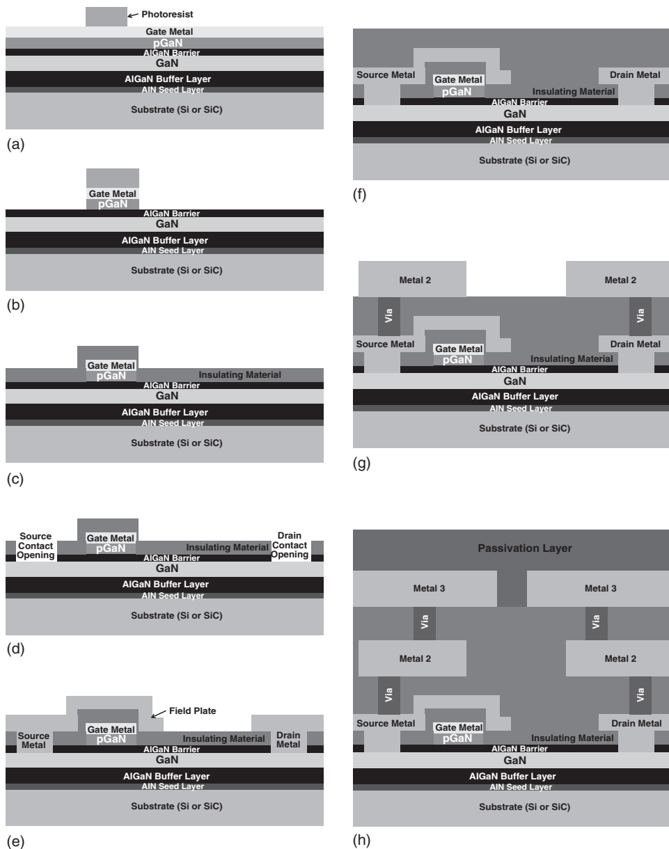
Figure 1.16 A typical process for fabricating an enhancement-mode GaN HEMT (not to scale) [24,25]. The process steps are as follows: (a) Deposit gate metal and define gate pattern using photoresist as a protecting layer. (b) Etch the gate metal and pGaIn crystal. (c) Deposit insulating material. (d) Create contact openings to source, drain, and gate (gate contact not pictured). (e) Deposit first aluminum metal layer and define metal pattern. (f) Deposit interlayer dielectric. (g) Cut vias between metal layers, form tungsten via plug, deposit and define second aluminum metal layer. (h) Deposit and define third aluminum layer and deposit final passivation layer
