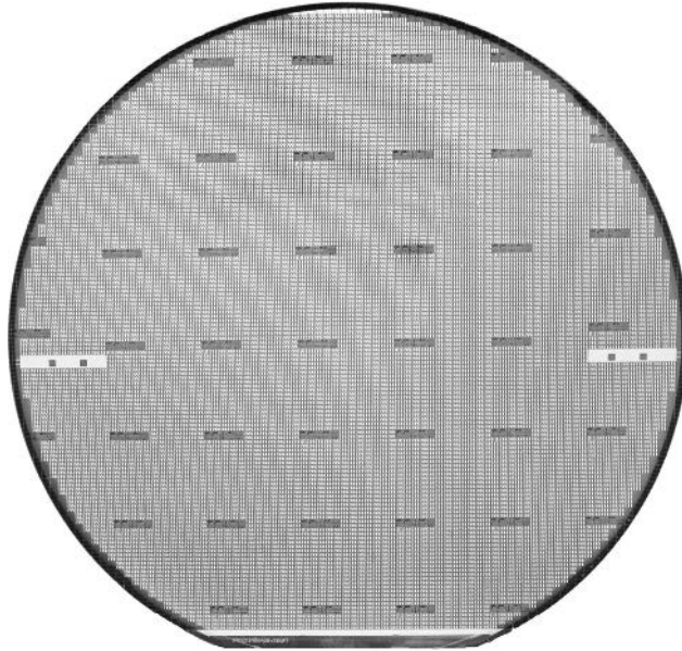
Figure 1.19 A completed 150 mm diameter enhancement-mode GaN HEMT wafer
